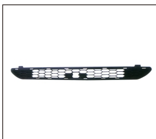
FRONT BUMPER GRILLE XLE 901G.TY05024BA OE:53112-0R110
